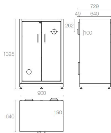
AC 900/130 S
