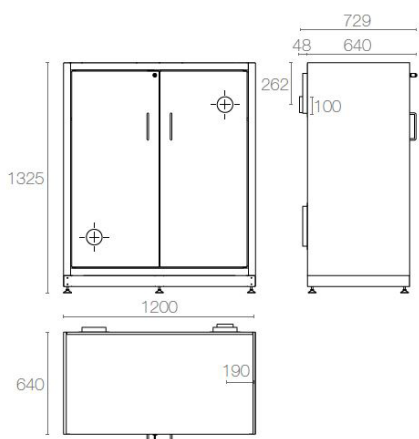
AC 1200/130 S
